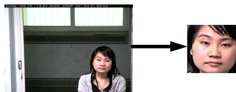
Figure 4. Face detection.
